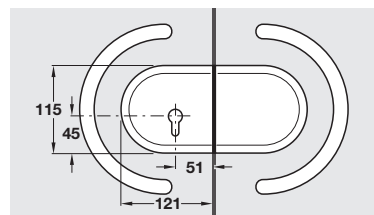
Cut out for lock and counter case are the same
