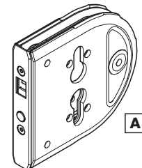
Use wall profile, seal and strike plate with lock, for locking to jamb or wall: single sliding door applications
