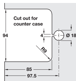
Cut out for lock and counter case are the same
