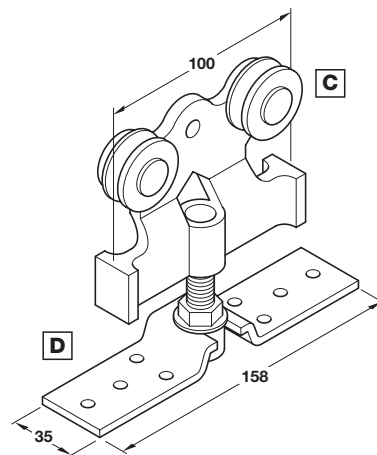
Side fixing
