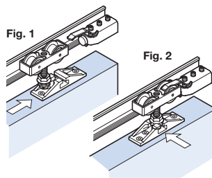
Fig. 1 - Side mounting Fig. 2 - Front mounting
