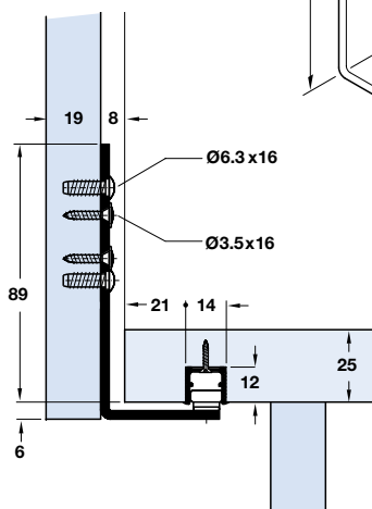
Concealed sliding door gear components Panels move across face of units
