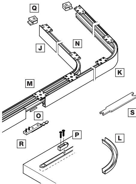
HAWA-Aperto 40/F parallel stacking area
