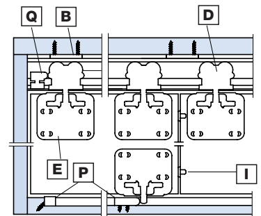
HAWA-Aperto 40/F parallel stacking area
