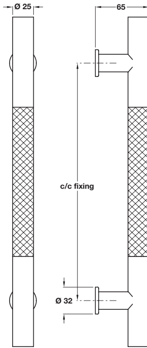
Example: Bolt through fixing
