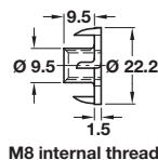
M8 internal thread
