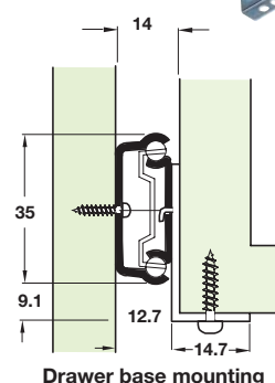
Drawer base mounting
