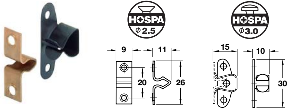
Spring catch 15 x 10 x 30 mm
