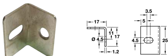
D Angle bracket
