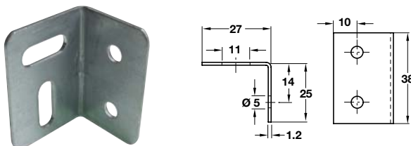
C Angle bracket
