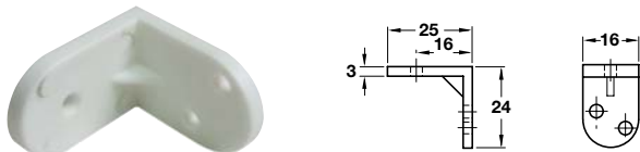
B Angle bracket
