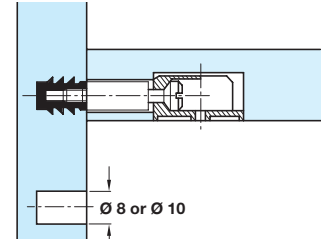
Connecting bolt with M6 thread for use in dowel or sleeve for push-fit or press-fit fastening in \varnothing 8 or \varnothing 10 mm hole
