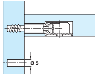
Connecting bolt with special thread for direct installation in \varnothing 5 mm hole
