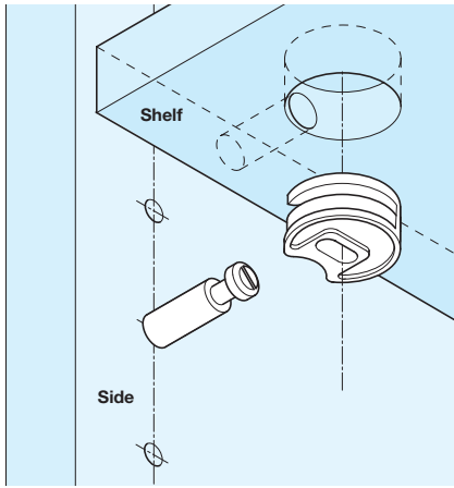
Connecting bolt with special thread for direct installation in \varnothing 5 mm hole
