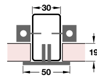
Flush fitted panel between columns
