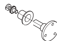
Variofitting knob mount with 7 mm square spindle, for fitting knobs provided by customer; page 110
