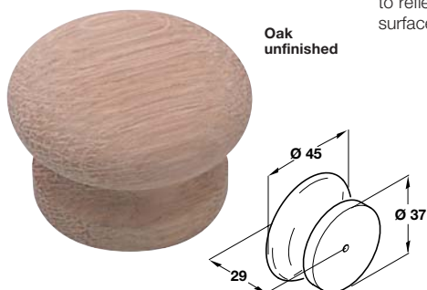
A Knob, Ø 45 mm
