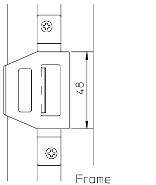
Horizontal Section
