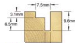
Diagrams of how Aquamac Weatherseal is fitted
